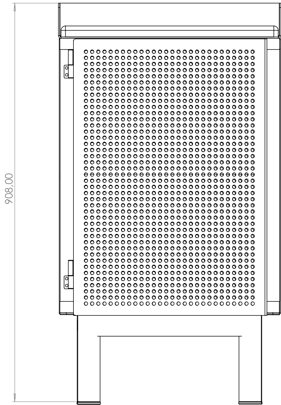
FRONT VIEW
