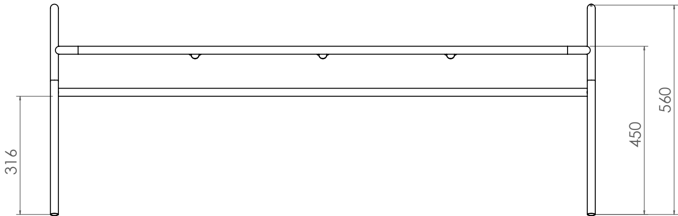
FRONT VIEW
