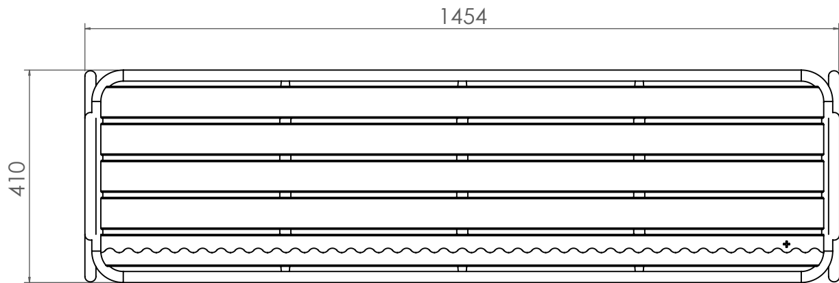
TOP VIEW
