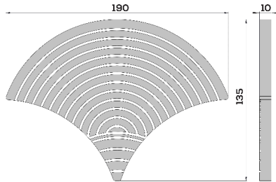
Line Drawing (mm) Variation in size can be expected
