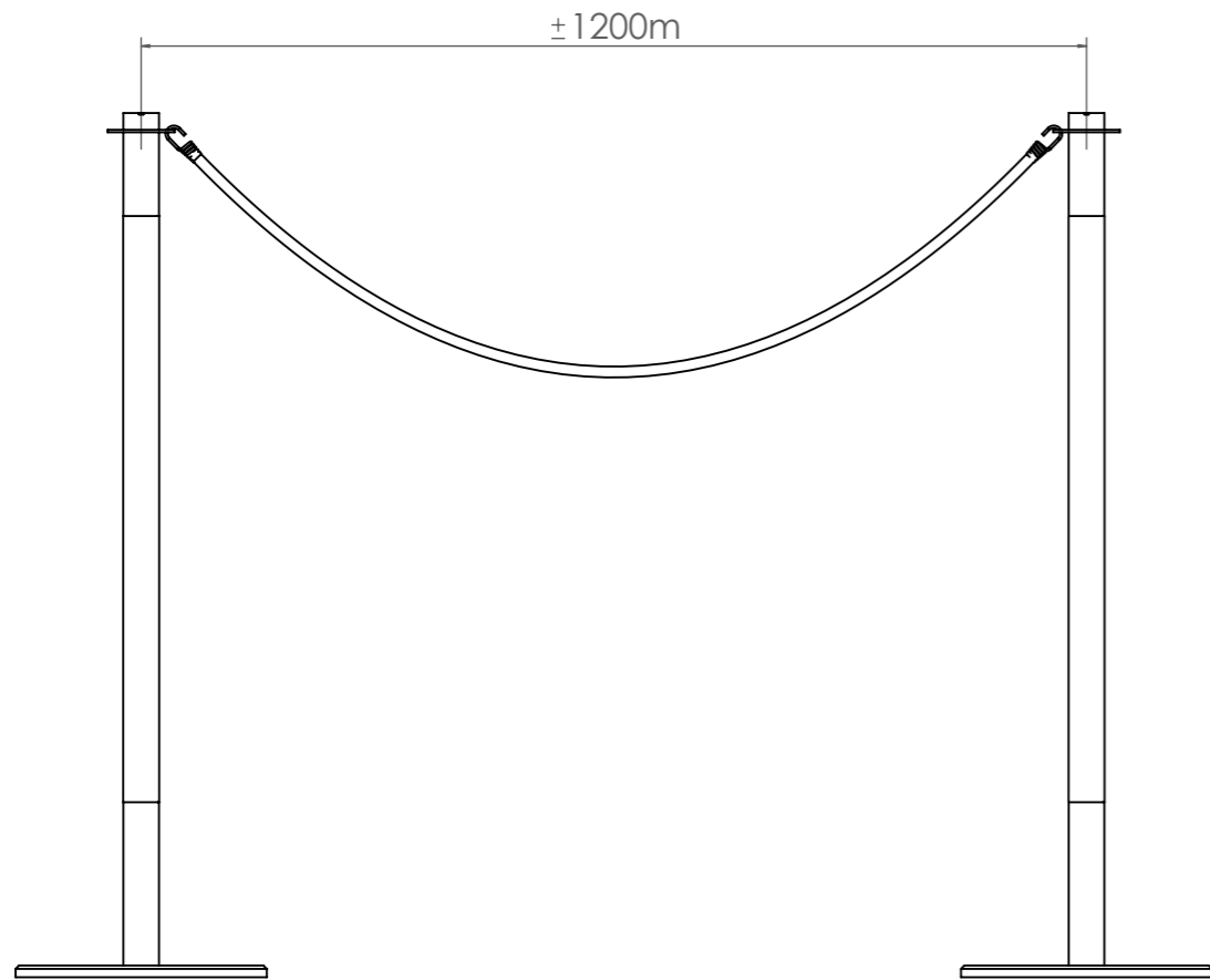
FRONT VIEW
