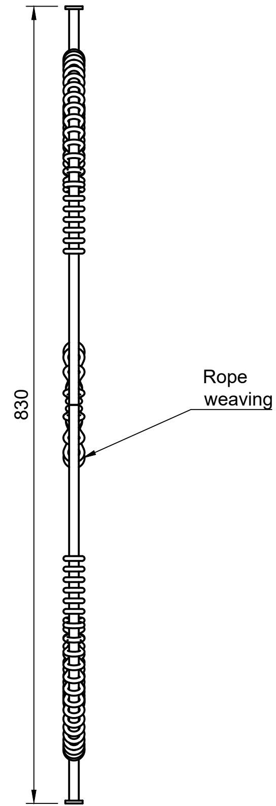
SIDE VIEW
