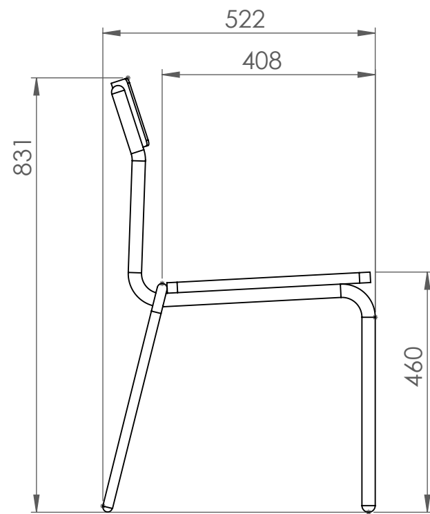
SIDE VIEW
