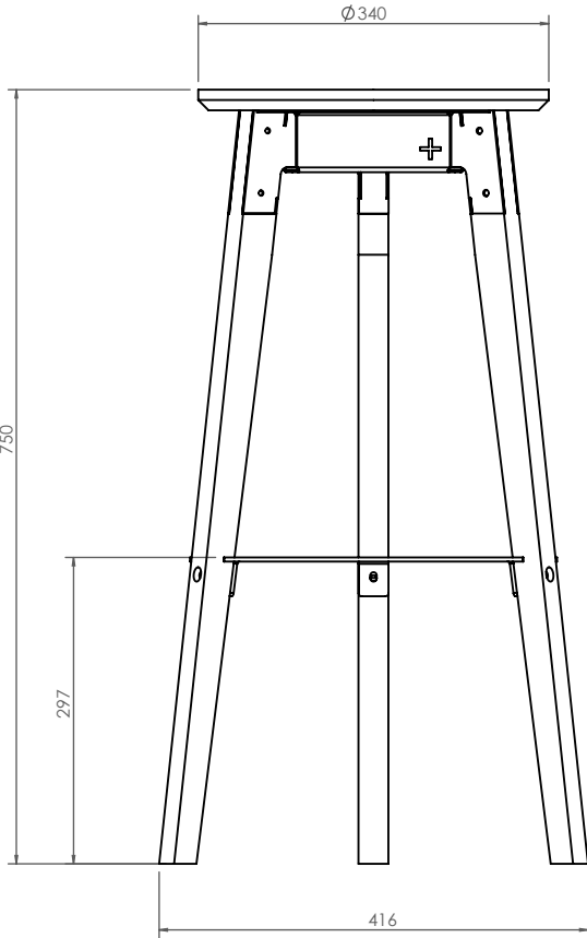
FRONT VIEW
