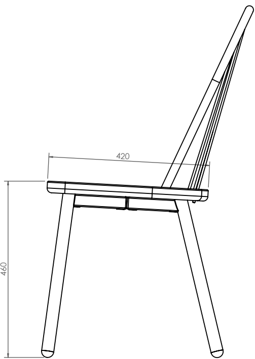
RIGHT VIEW
