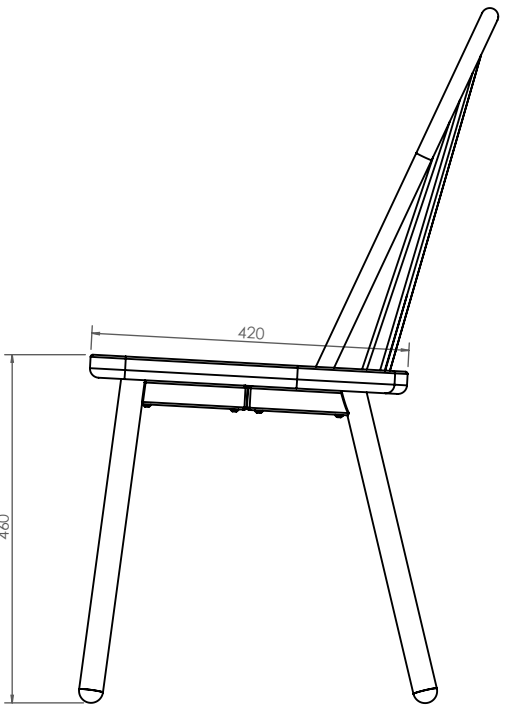
RIGHT VIEW
