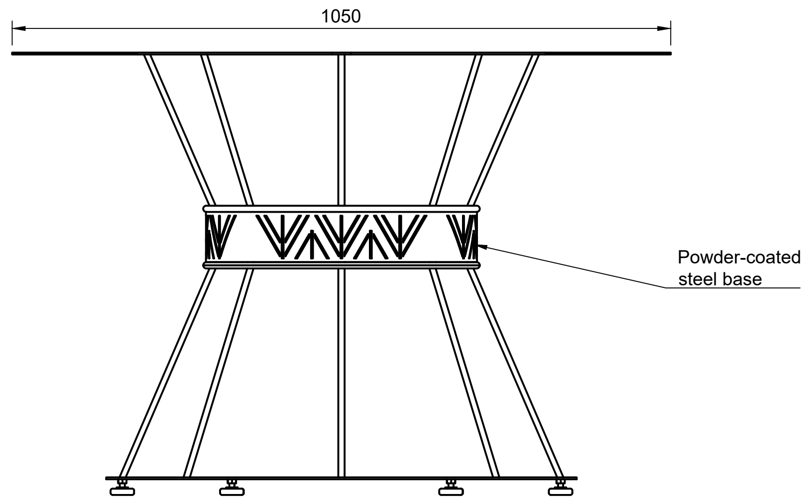
FRONT VIEW
