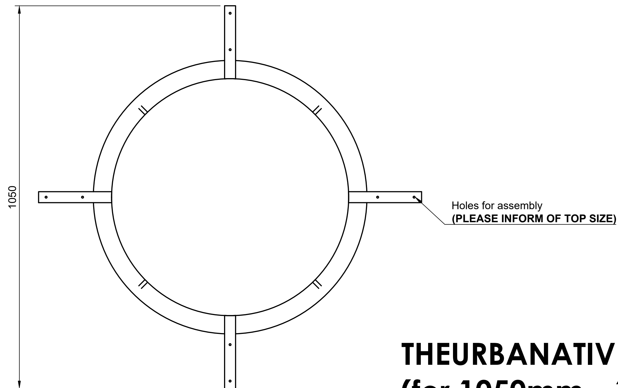
TOP VIEW
