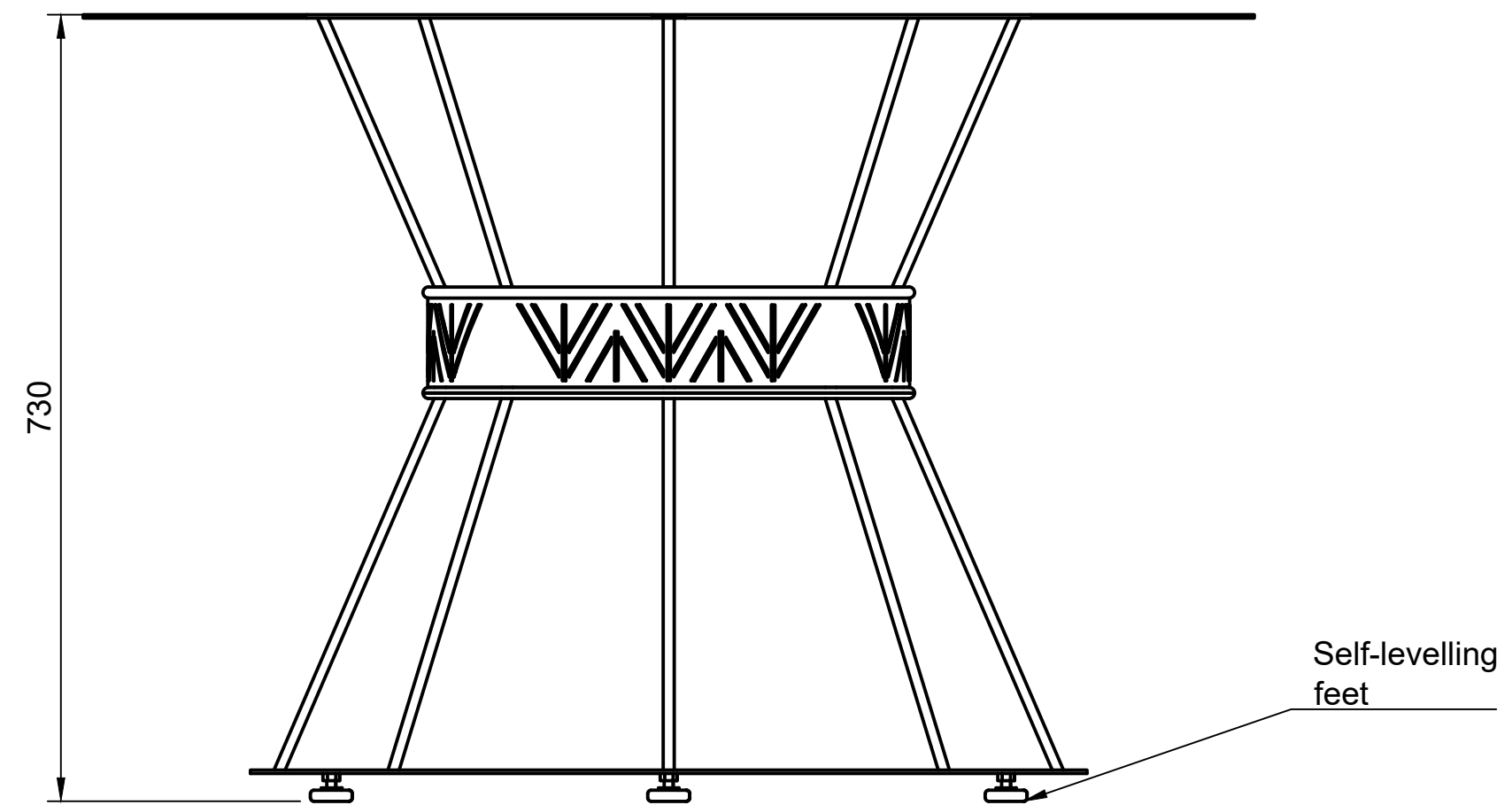
SIDE VIEW
