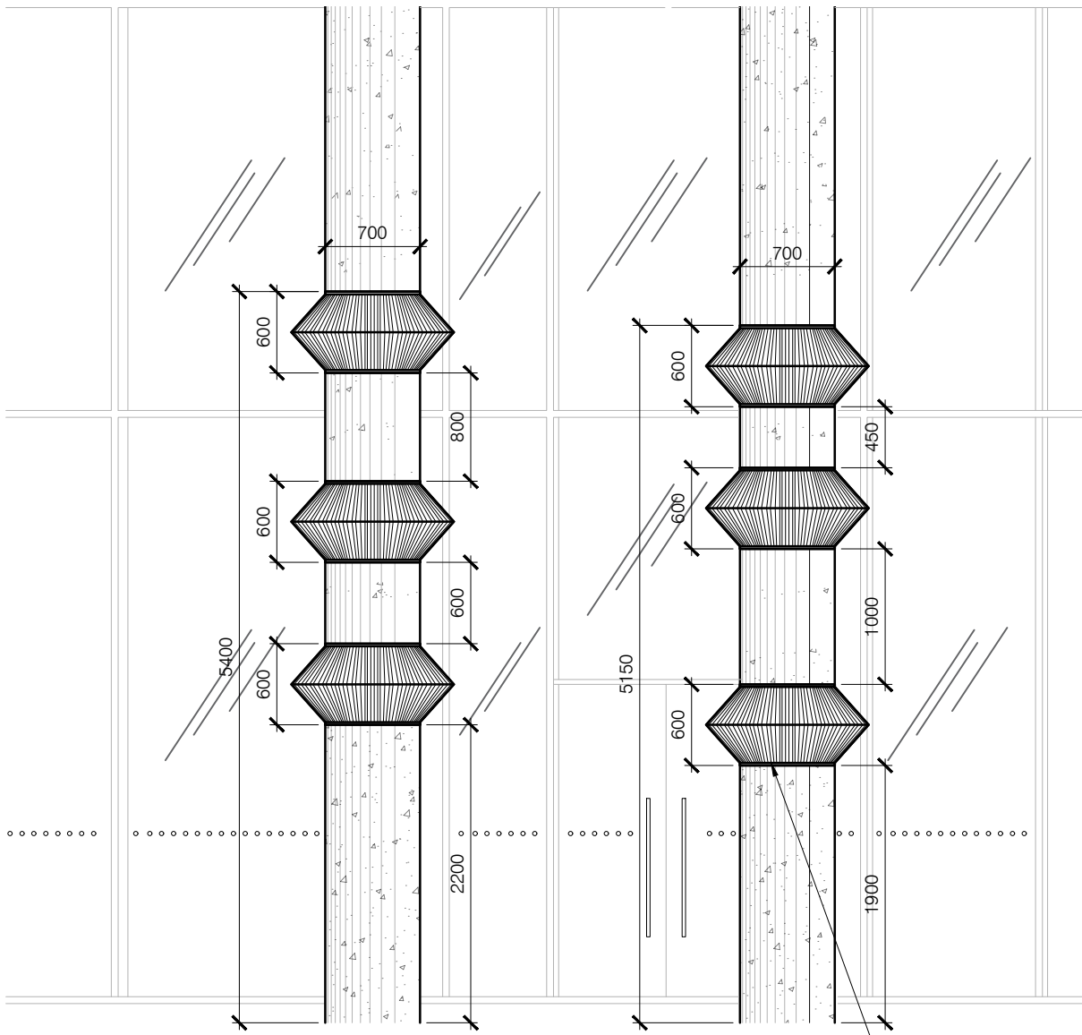
Decorative Column Collar Elevation Scale 1:50
