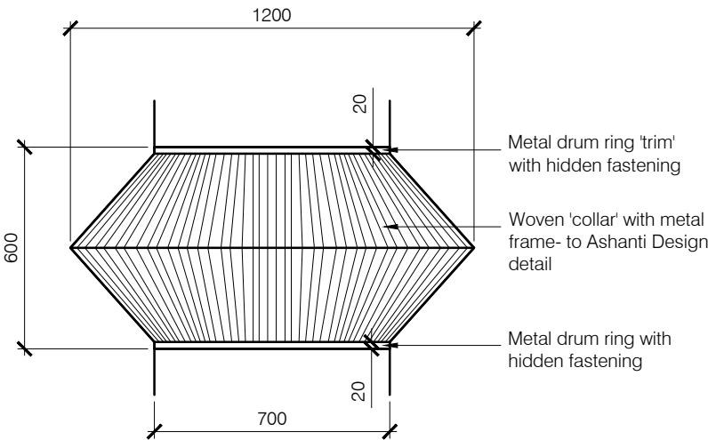
Decorative Collar Detail Scale 1:20
