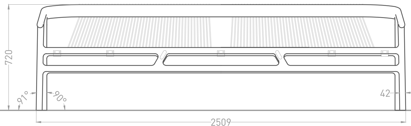
Front View Scale 1:16 on A4
