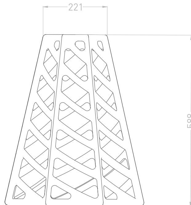
Right View Scale 1:8 on A4
