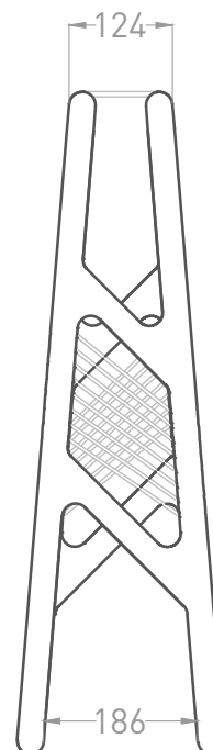
Side View
