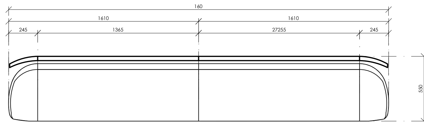
F2, Dinner Bench, Plan, Scale 1:20
